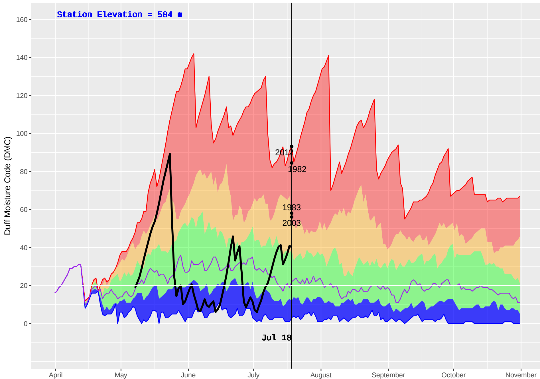
SIERRA (117) : Historical (1981–2016) and Current (2018) Daily Duff Moisture Code (DMC)
